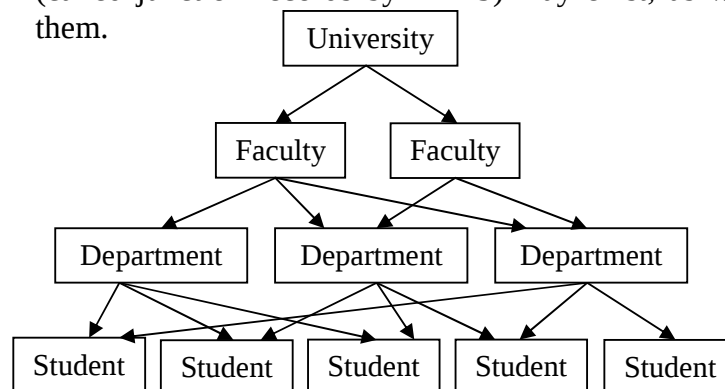
Fig. 4.2: Network Data Structure
